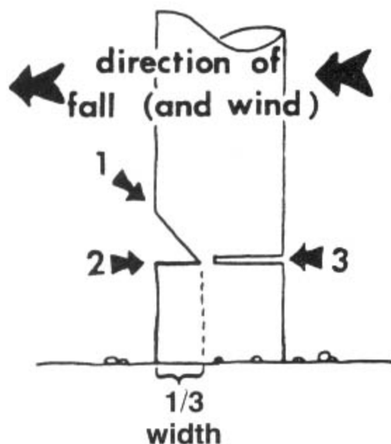
Chainsaw felling; note sequence of cuts.
